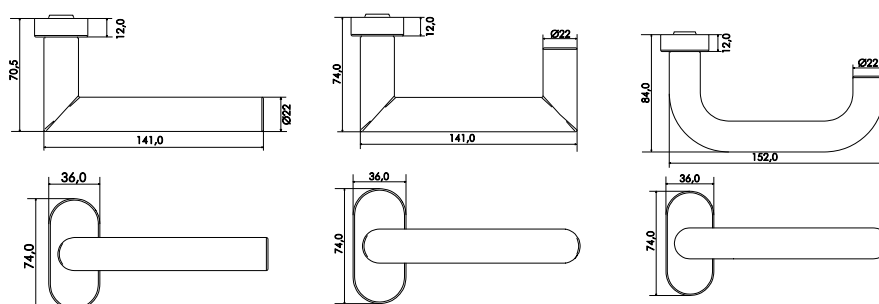
Oval rosette mechanical side
