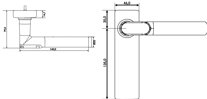
Short plate electronics side
