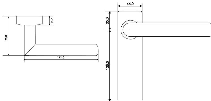
Short plate mechanical side
