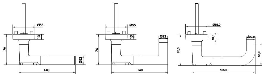
Circular rosette electronics side and handle versions
